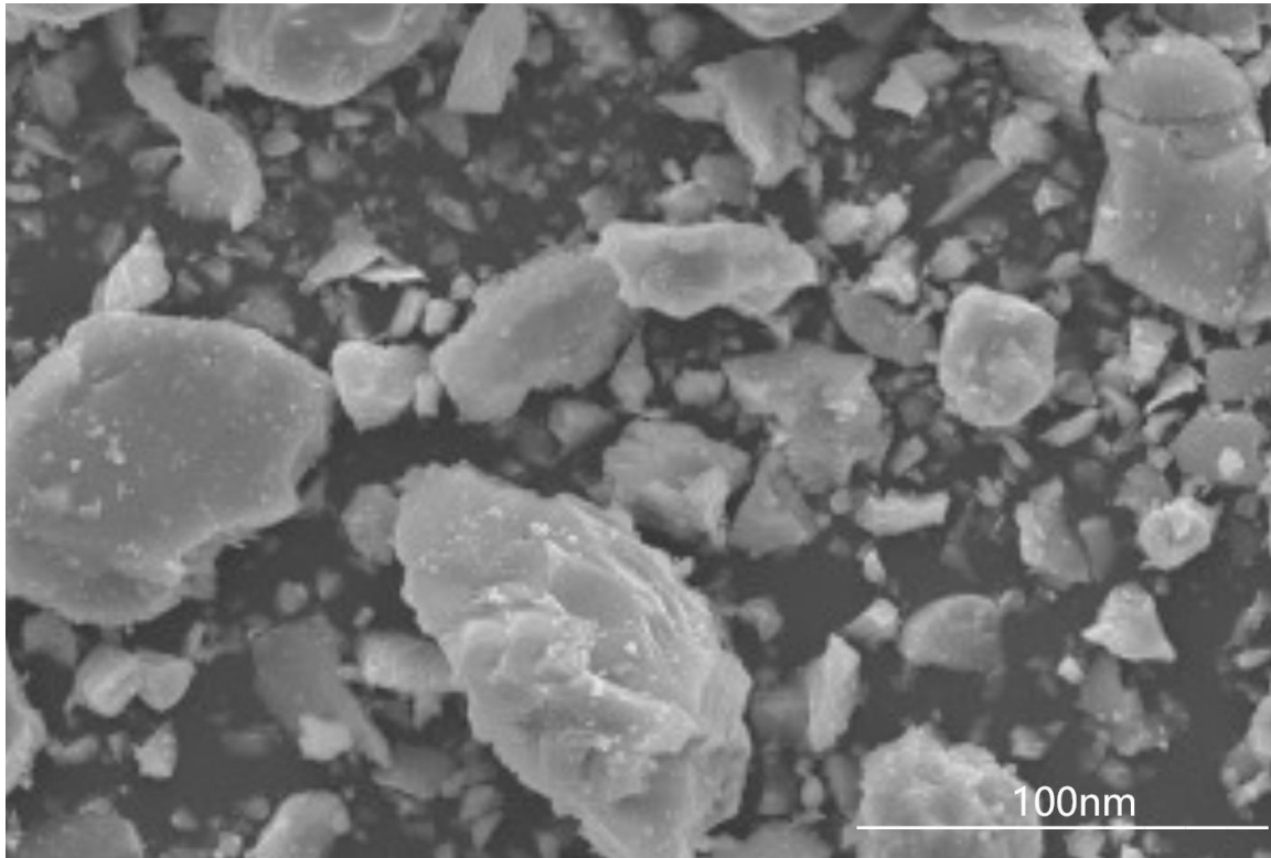
SEM Image (Sulphur nano powder):
