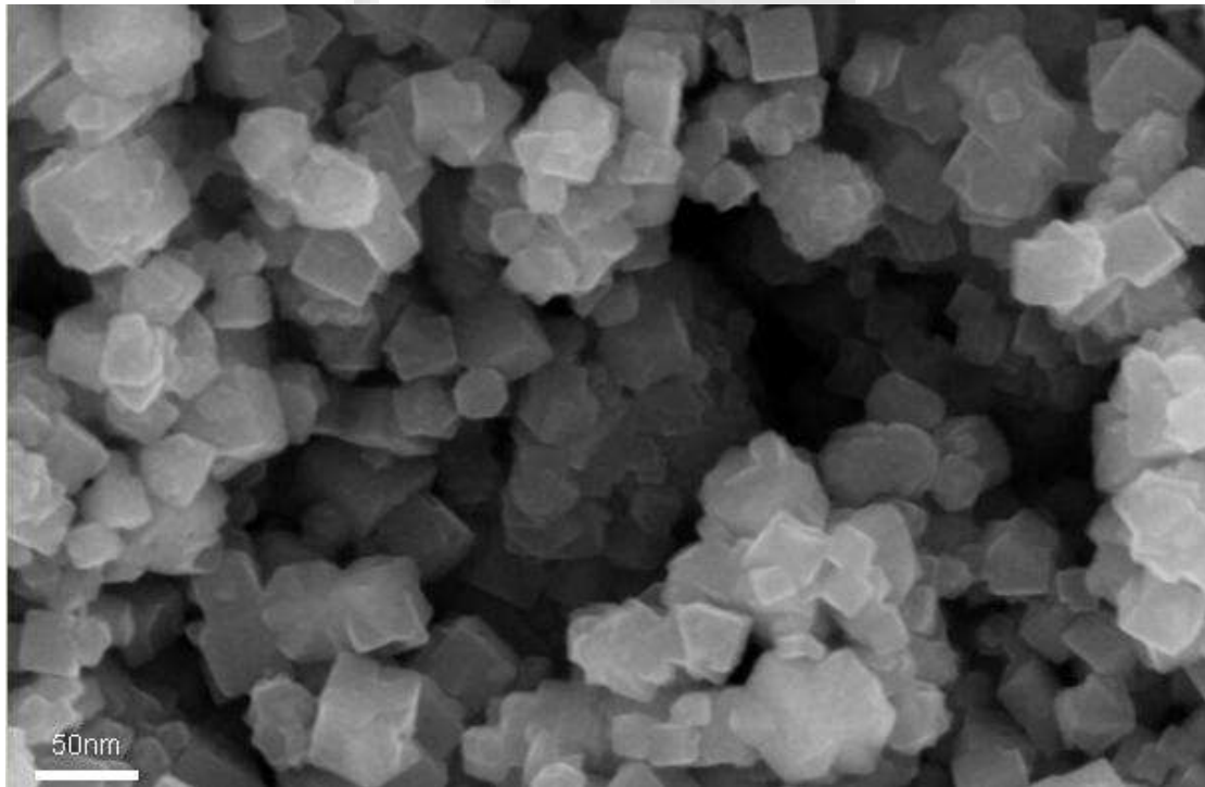
SEM Image of Fe 3 O 4 nano Powders
