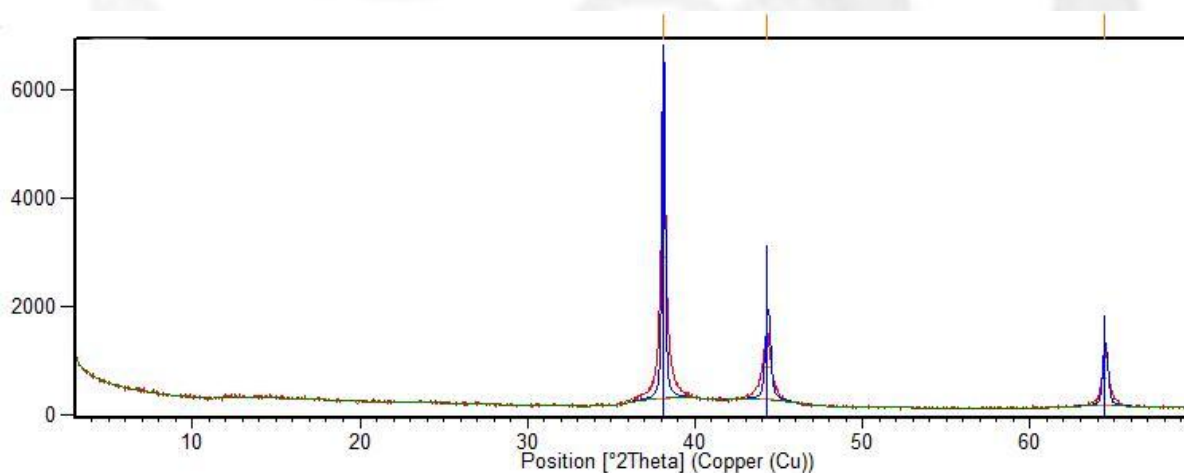
XRD of Silver Nano Powders
