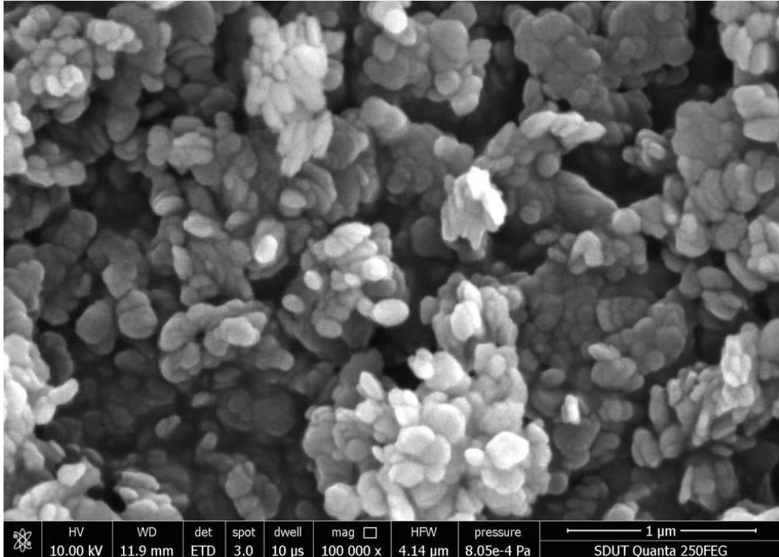
SEM Image of Boron Nitride nanopowder
